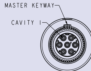
6-7 LAYOUT
