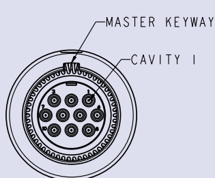
7-10 LAYOUT
