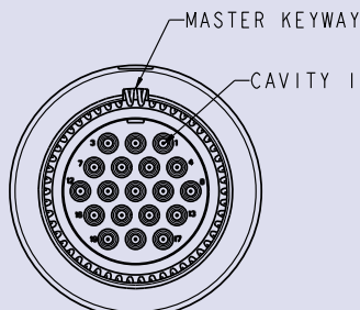
9-19 LAYOUT
