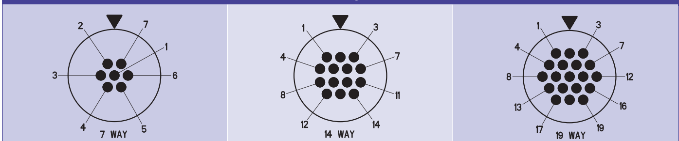
Face View, Pin Contacts. Cavity identification numbers are for reference only; they do not appear on connectors.
