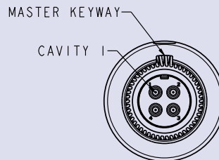
6-4 LAYOUT
