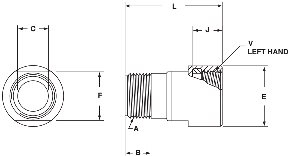
10-350695-XX( ) adapter
