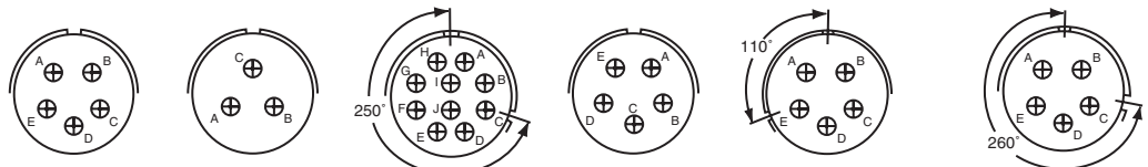
250° Rotation of 18-1
